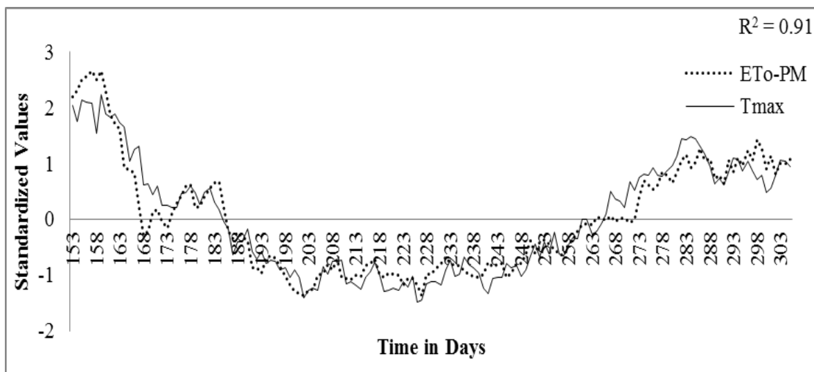
Fig 2: Dependency of ET 0 -PM on Tmax at Daily time-scale for Junagadh (1992-2002)
