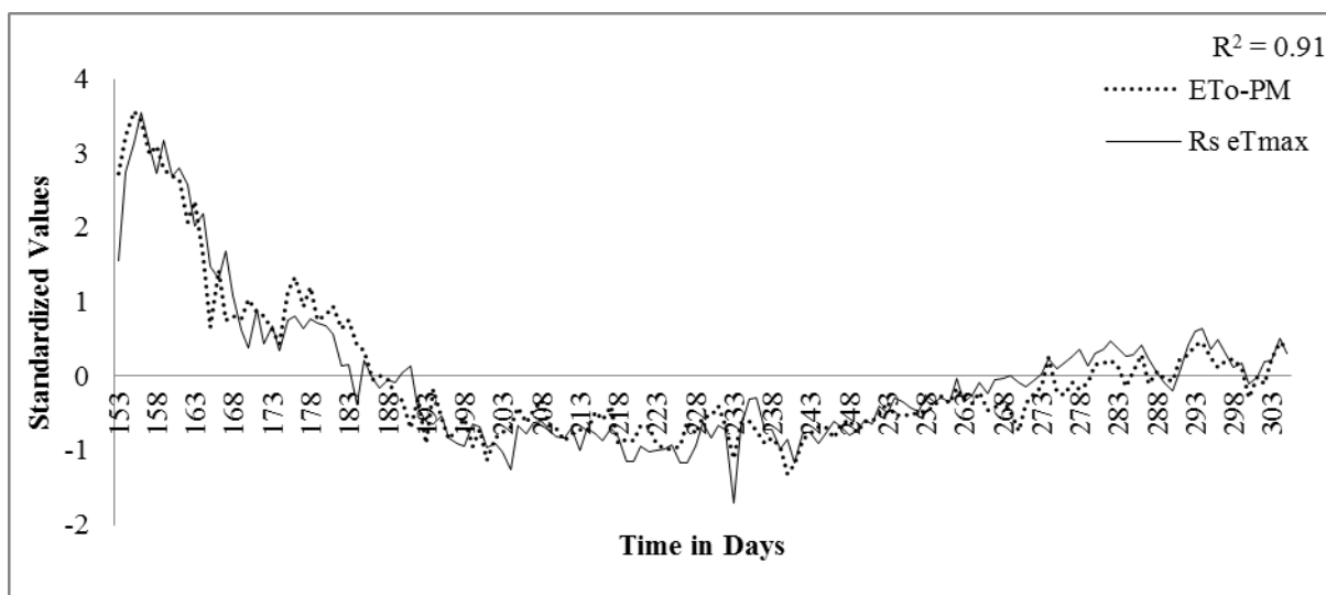
Fig 7: Dependency of ETo-PM on Rs eTmax at Daily time-scale for Amreli (1992-2002)
