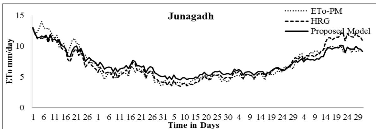
Fig 8: Performance of Hargreaves method and Proposed model for daily time steps in validation period (2003-2012) for Junagadh
